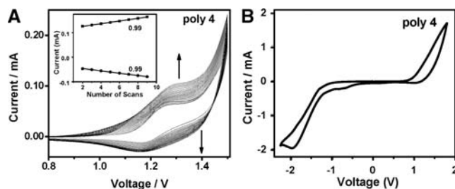
Figure 4. Electropolymerization of 4 from acetonitrile solution at a scan rate of 100 mV/s. Inset picture: Linear relationship of increase in current with number scans (A). Cyclic voltammogram of poly 4 (B).
